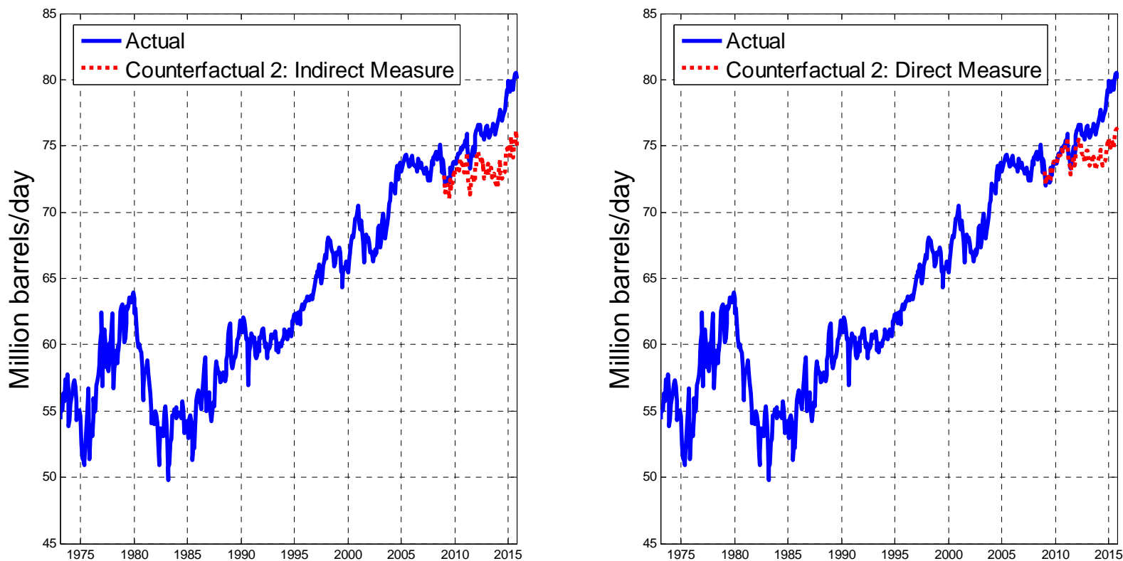
Figure 9. Alternative Counterfactuals for World Oil Production in the Absence of the U.S. Fracking Boom
