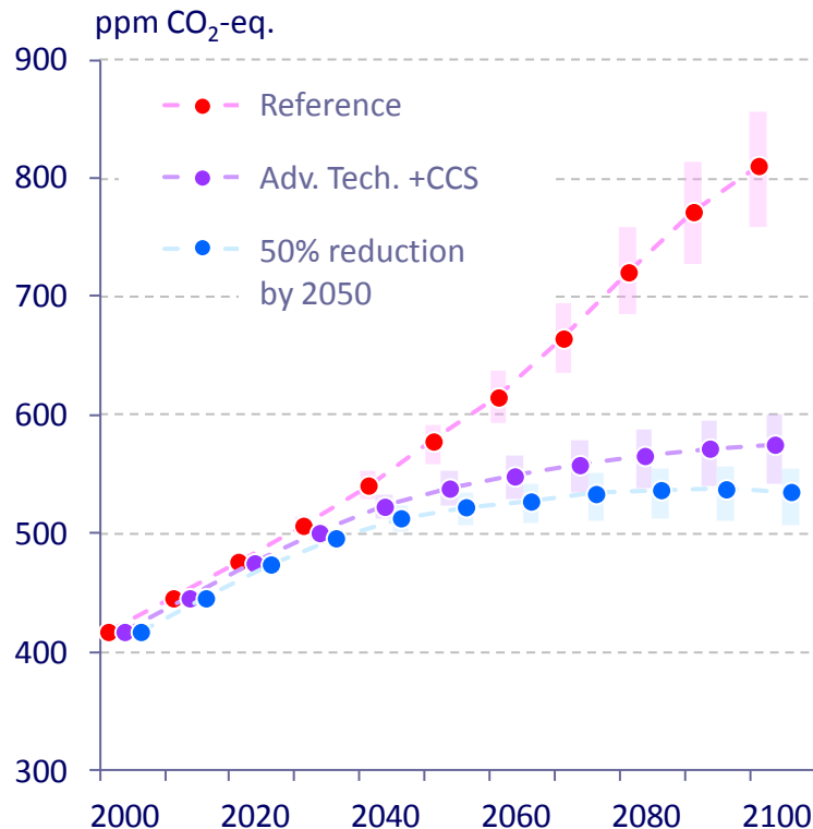
GHG concentration
