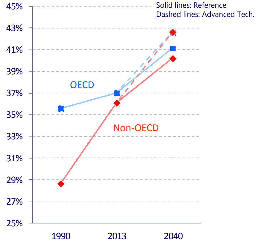
Thermal efficiencies of coal-fired power plants
